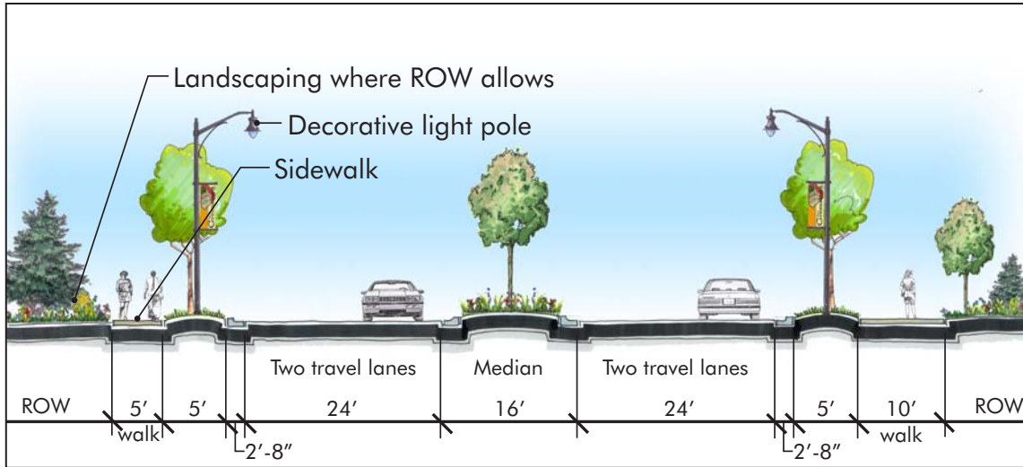
▲ Figure E.3: Proposed Typical Cross-Section of Freeland Road West of SR 3
