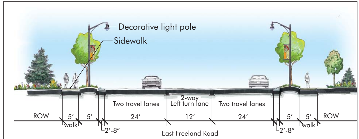
▲ Figure E.4: Proposed Typical Cross-Section of Freeland Road East of SR 3
